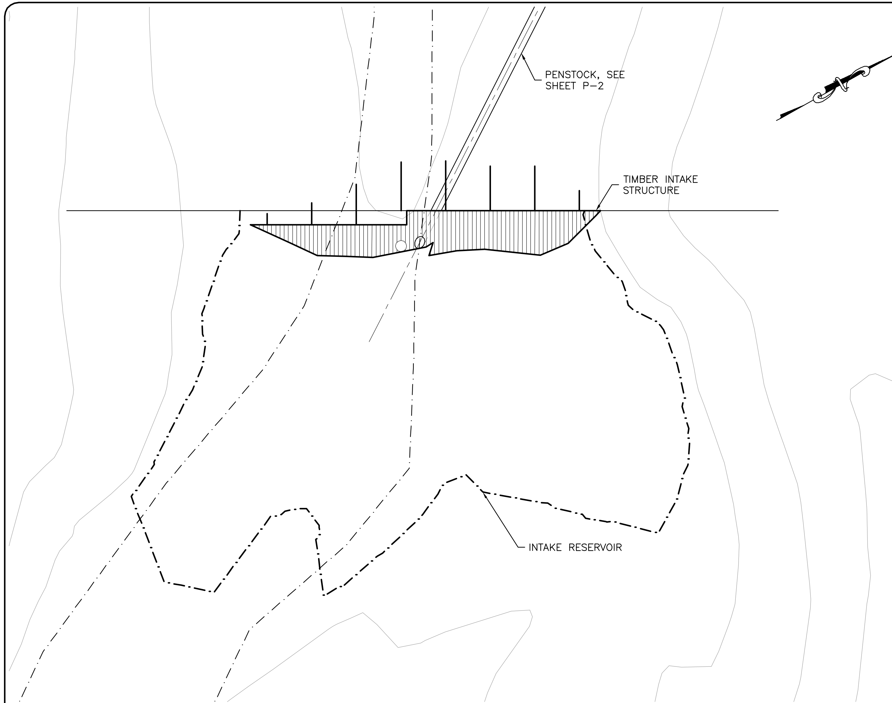
1 INTAKE PLAN SCALE: 1" = 10'
